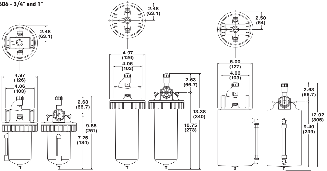
"W" 16 oz size bowl Inches (mm)
